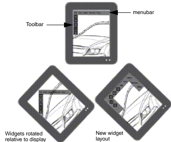
Figure 11. Not only do UI graphics have to be able to draw at arbitrary orientations in a RUI, perimeter widgets like menubars and toolbars may have to adopt different layout schemes depending on the rotation.
